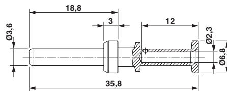
Dimensional drawing
